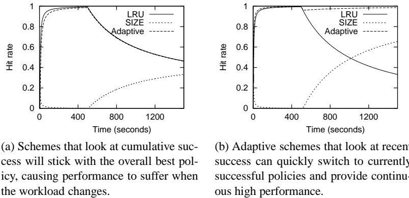
Figure 4: Hit rate for a synthetic workload that changes after 500 seconds.
